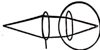
Convex lens
