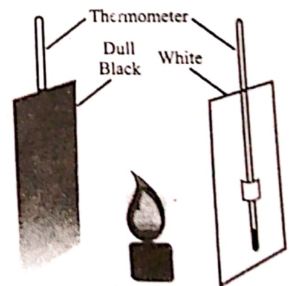
Figure 9.16: A comparison of absorption of radiation.
